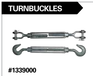
Galvanized Turnbuckles Hook + Hook & Jaw + Jaw shown. Also available Eye + Eye
